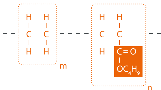
Fig. 4a: Molecular structure of EBA copolymers
