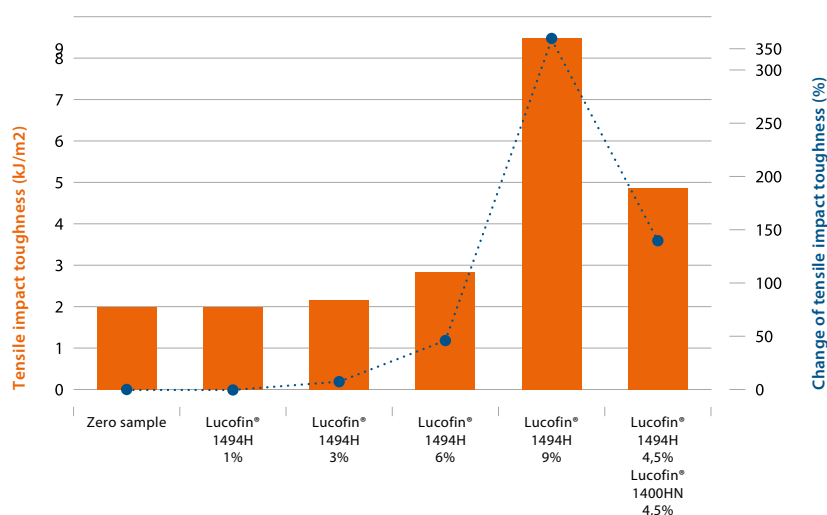
Fig. 12: Improvement of mechanical properties of a PP/EVOH (PP: 86 %, EVOH: 14%) blend by adding Lucofin® 1400HN/Lucofin® 1494H- tensile impact toughness
