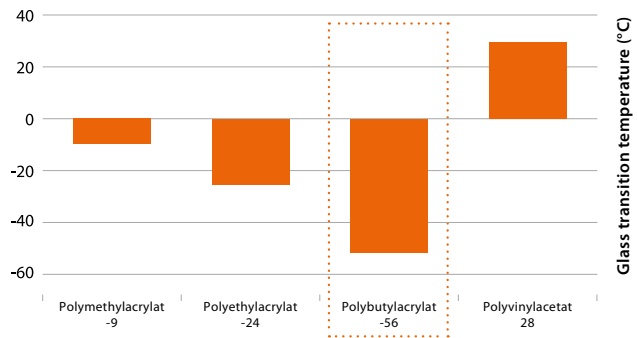
Figure 9: Glass transition temperature of some polar ethylene copolymers
