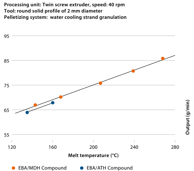
Figure 10: Output of HFFR compounds based on EBA/ATH Compound and EBA/MDH as a function of melt temperature
