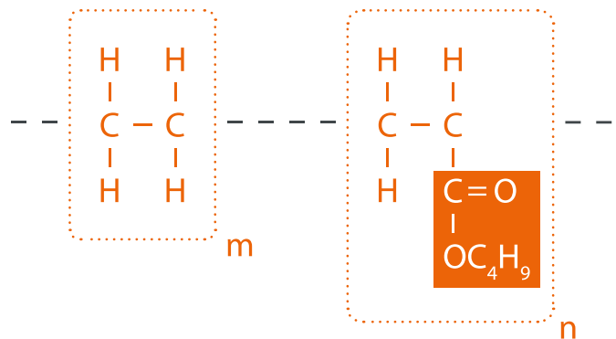
Figure 1: Molecular structure of ethylene butyl acrylate (EBA)
