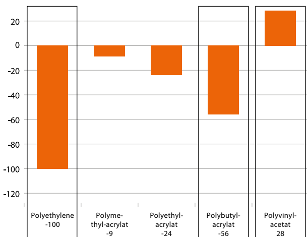
Figure 5: Glass transition temperature of polyethylene and some polar ethylene copolymers
