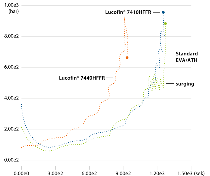
Figure 11: Rheology curve for Lucofin® 7410HFFR, Lucofin® 7440HFFR and for a standard EVA/ATH compound
