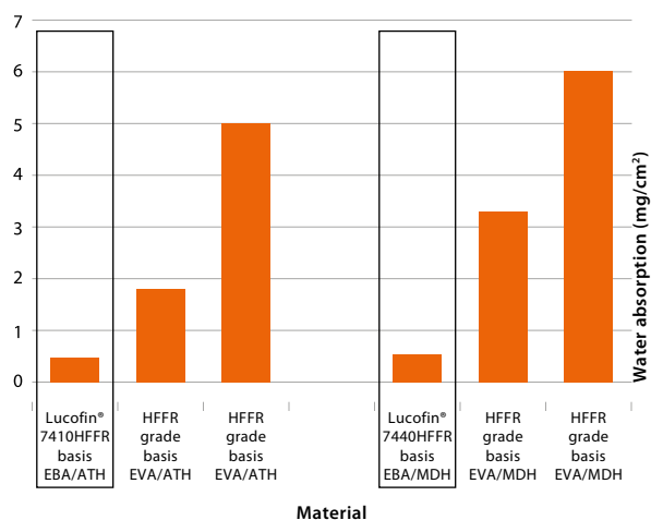
Figure 2: Water absorption of various HFFR grades
