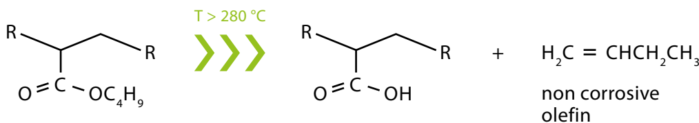
Figure 9: Thermal decomposition of EVA and EBA at different temperatures yielding corrosive and non-corrosive by-products, respectively
