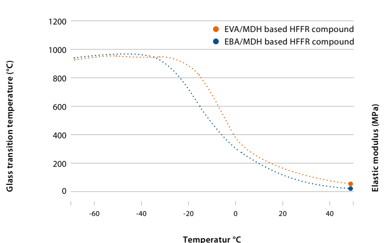
Figure 6: Dynamical Mechanical analysis (DMA) of HFFR compounds based on EVA/MDH and EBA/MDH
