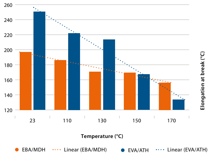
Figure 8: Elongation at break of HFFR compounds based on EBA/MDH and EVA/ATH as a function of storage temperature
